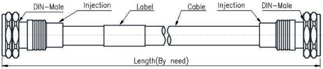
1/2" flexible Jumper Assembly, DIN type male to DIN type male
